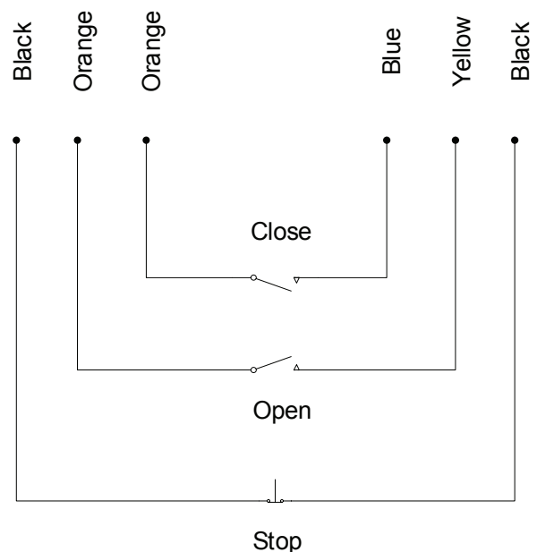
CI-KXS & CI-KFS Schematic
