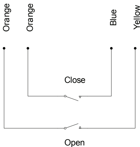
CI-KX & CI-KF Schematic
