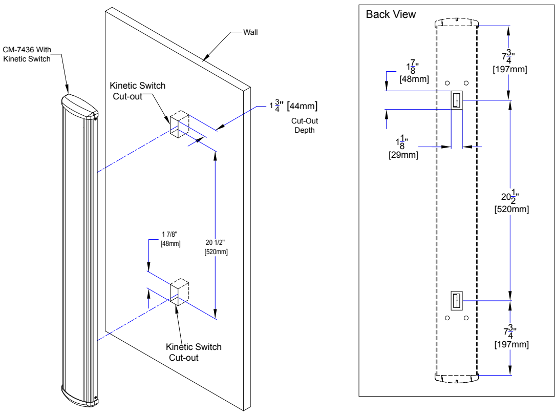
Figure 4.5 Kinetic Wall Mounting
