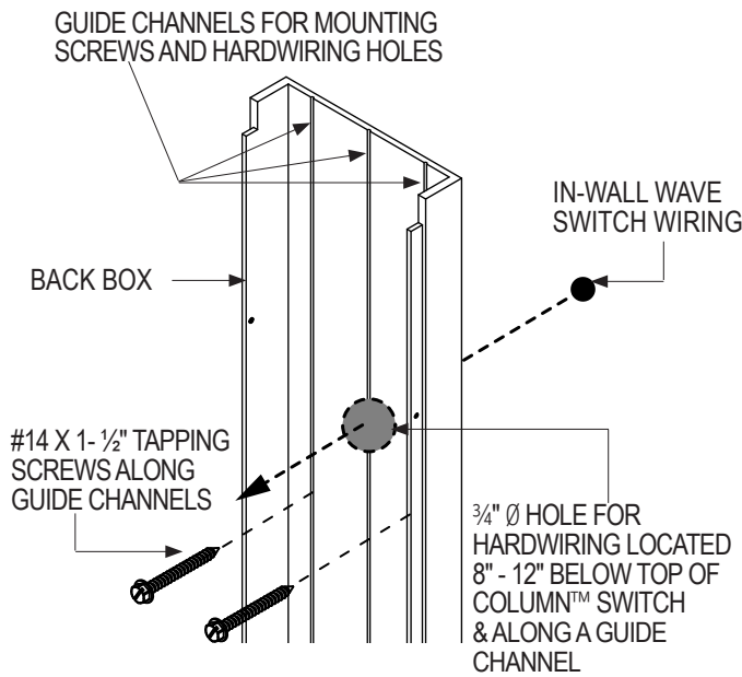
Figure 4.3 Guide Channels
