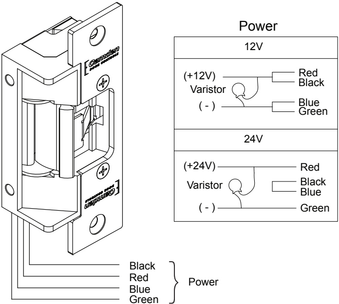
Figure 8.1 Connections for CX-ED2079
