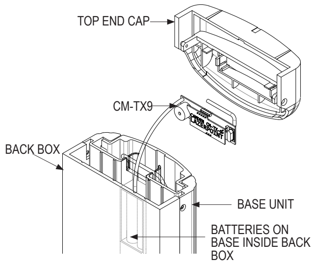
Figure 4.5 Lazerpoint RF
