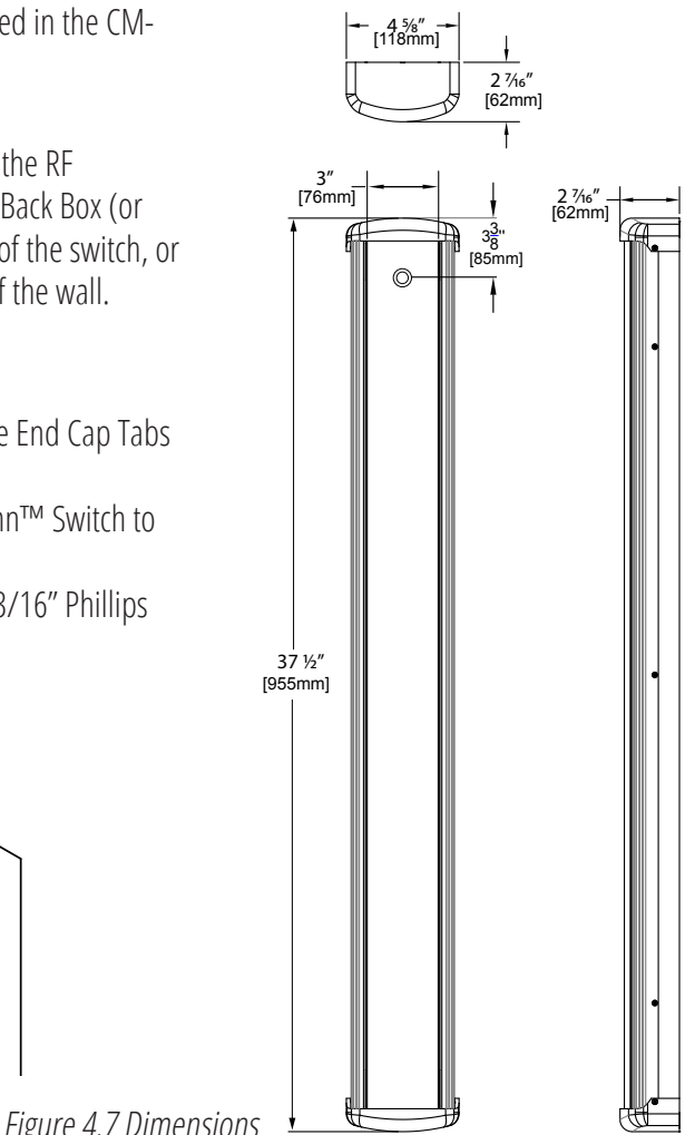
Figure 4.7 Dimensions
