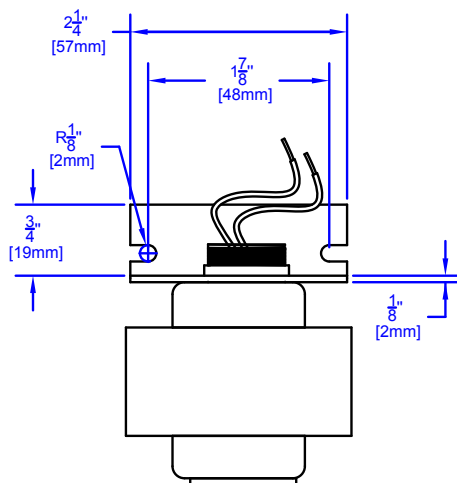
CX-TRN - 2024 - 24V AC 20VA NIPPLE MOUNT TRANSFORMER
