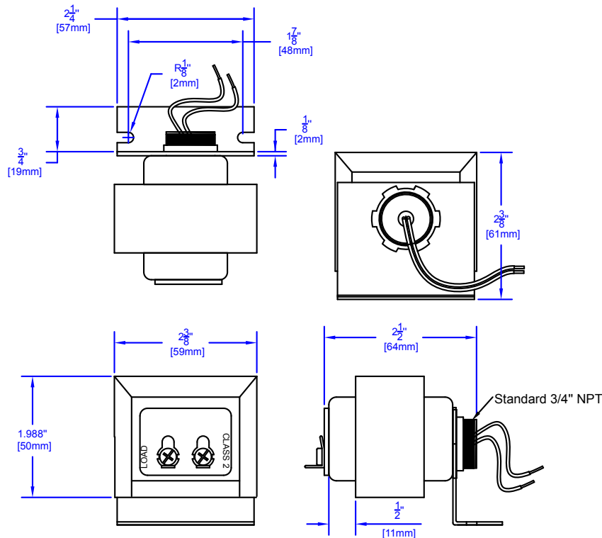
CX-TRX - 4024 12VAC 36VA NIPPLE MOUNT TRANSFORMER.
