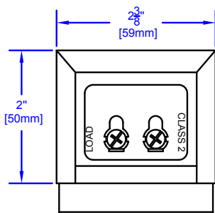
CX-TRX - 2012 12VAC 20VA NIPPLE MOUNT TRANSFORMER.
