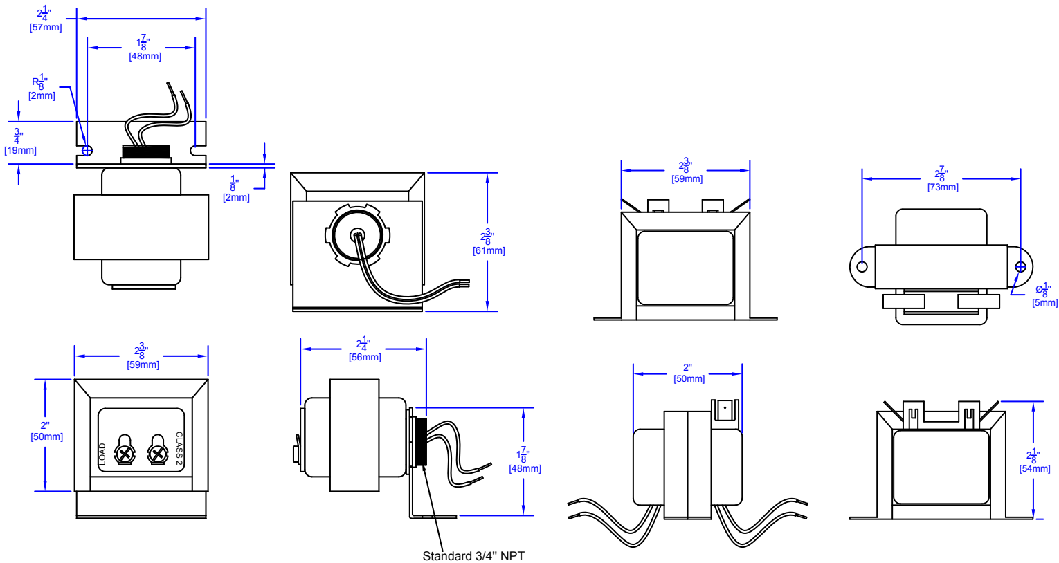
CX-TRX-2024 - 24VAC, 20VA STANDARD MOUNT TRANSFORMER
