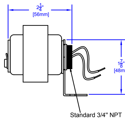
CX-TRX - 2012 12VAC 20VA NIPPLE MOUNT TRANSFORMER.
