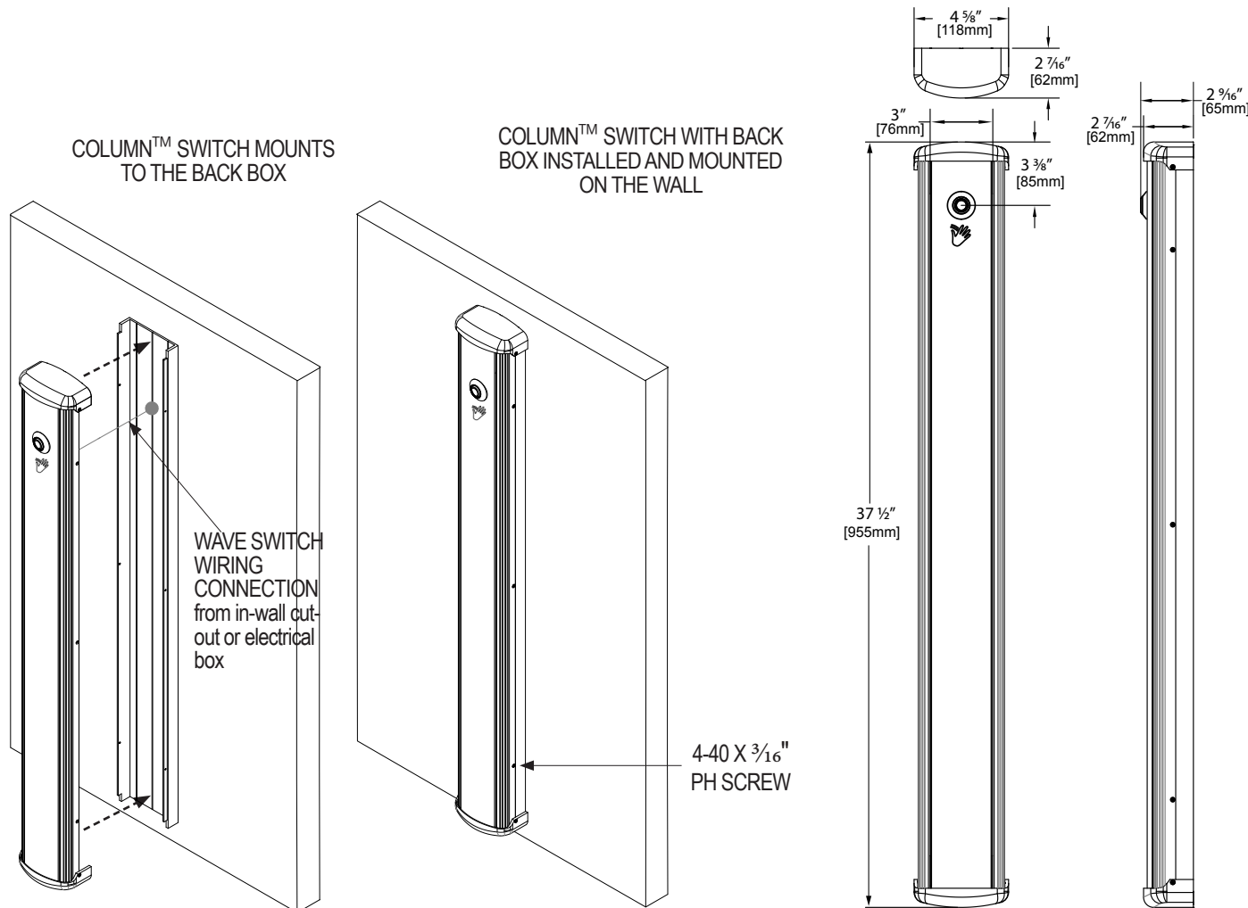
Figure 4.5 Installation
