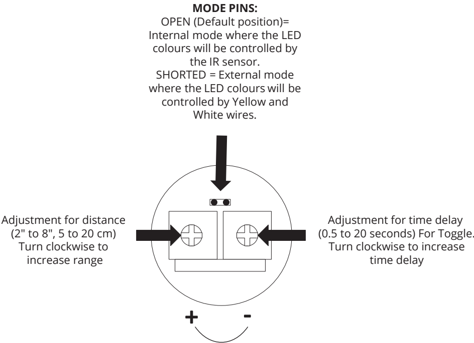
Figure 5.1 Configuration
